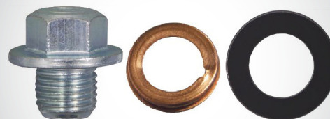
670-P61200430 M12x1,25x11 AV14 6420043A 12x17x3 6420043D 12x21x1,7
